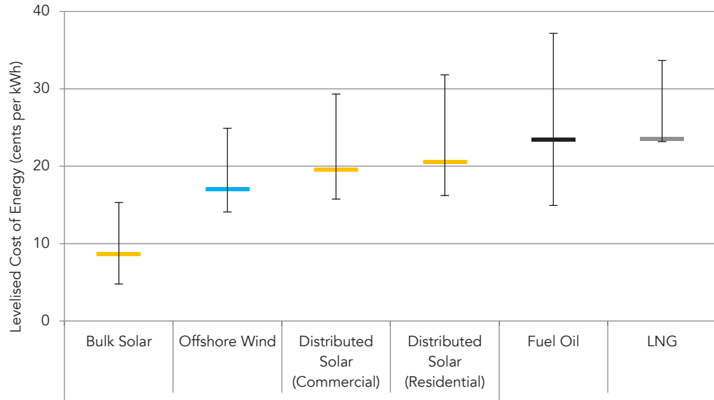
Figure 13 – Levelized energy costs calculated for this study, in 2017 dollars
