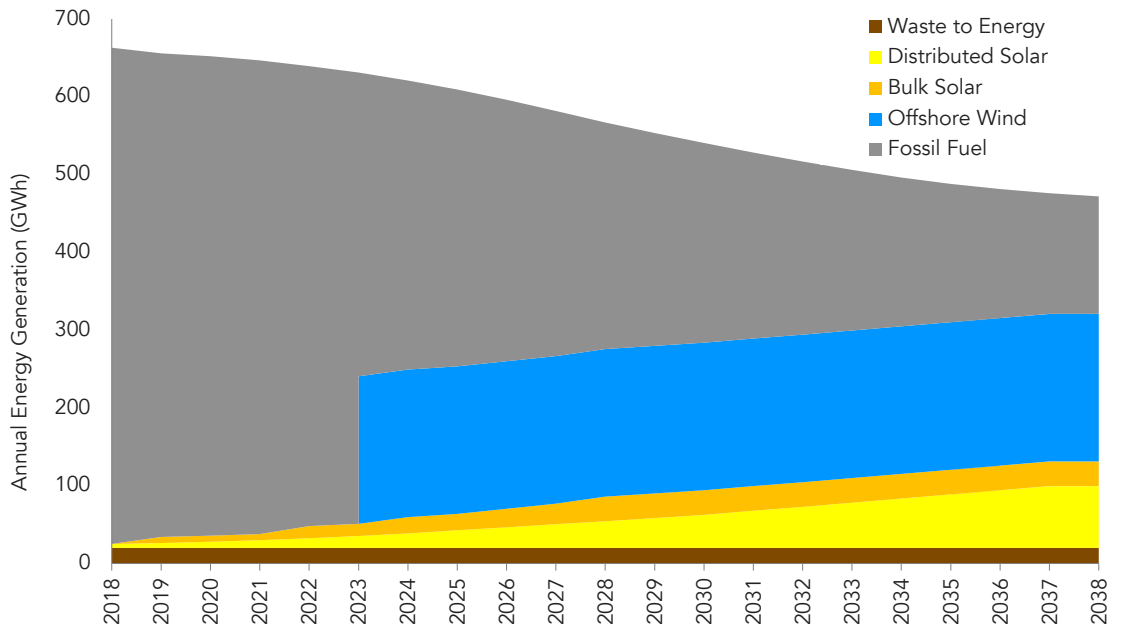
Bermuda’s changing energy mix in the optimum renewables scenario
